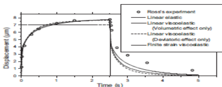
Figure 2 Curve fitting of the creep test data.
